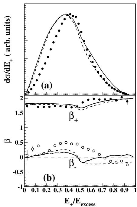
Figure 3. (a) SDCS = d\sigma/dE_+ , energy in units of the 100 eV excess energy. (b) \beta -parameter of the k_+ and k_- momenta. The dots are the experimental data, the solid and dashed curves show 3C calculations in length and velocity form, respectively.
