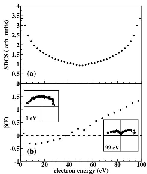
Figure 2. (a) Electron energy distribution or single-differential cross section ( d\sigma/dE_1 ). (b) \beta -parameter of one electron from helium double ionization at 179 eV photon energy. The insets show the DDCS d^2\sigma^2/(d\Omega dE) at E = 1 and 99 eV in polar coordinates.
