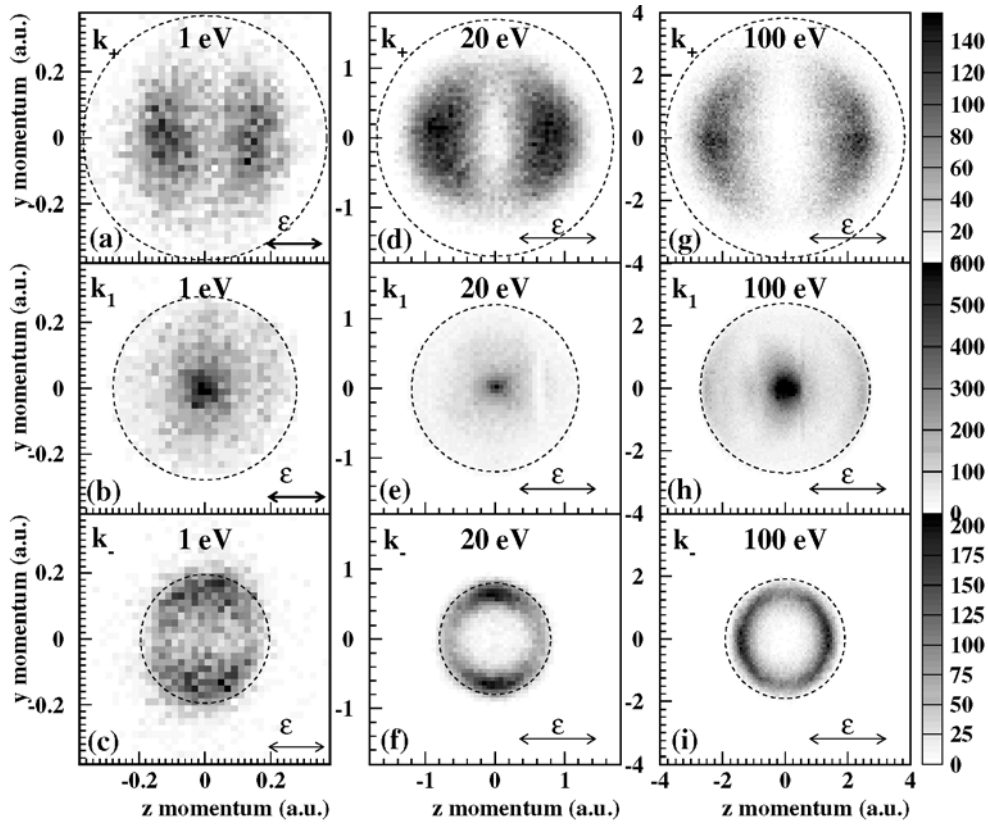
Figure 1. Density plots of projections of the momentum distributions from double ionization of He by three different energies, from left to right: data sets for 1, 20 and 100 eV above threshold. The data for 1 and 20 eV (left and middle column) are previous measurements, see also [2, 3]. The measurement at 100 eV above threshold is displayed in the right column. The z and y components of the momentum are plotted on the horizontal and vertical axes, respectively. The polarization vector of the photon is in the z direction and the photon propagates in the x direction perpendicular to y and z . The plots are projections onto the y - z plane with -0.1 < k_x < 0.1 au for the 1 eV data set, -0.2 < k_x < 0.2 au for the 20 eV data and for the 100 eV above-threshold measurement only events with -1 < k_x < 1 au are projected onto the plane. (a), (d), (g) Momentum distribution of the \text{He}^{2+} ion ( k_+ ) for 1, 20 and 100 eV above threshold, (b), (e), (h) electron momentum ( k_1 ) and (c), (f), (i) electron pair relative momentum (k_1 - k_2)/2 . The circle locates the maximum possible momentum in each coordinate at the respective photon energy.
